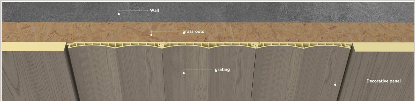
Decorative line board installation elevation drawing
